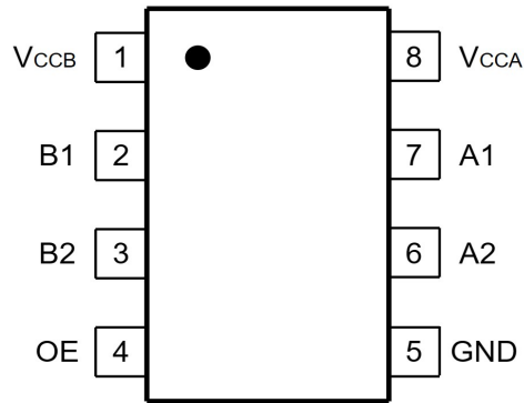
8-Pin TSOT23 Top View Fig.2 Pad definition of SC0102
