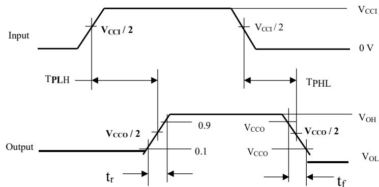
Figure 7-5. Voltage Waveforms Propagation Delay Times
