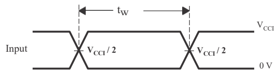
Figure 7-4. Pulse Duration
