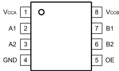
8-Pin MSOP Top View Pad definition of SC0102
