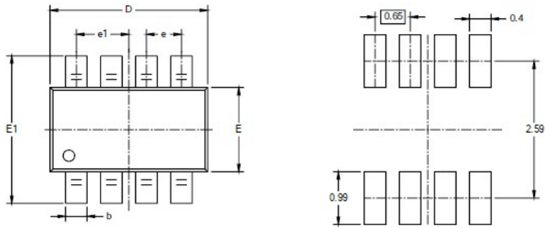
RECOMMENDED LAND PATTERN (Unit: mm)
