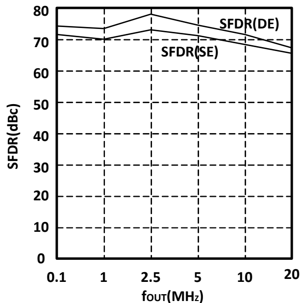
Figure 7. SFDR vs. f_{OUT} @ f_{CLK} = 100 MHz (Single-Ended and Differential-Ended)
