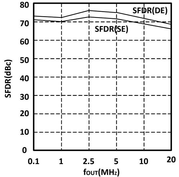
Figure 11. SFDR vs. f_{OUT} @ f_{CLK} = 100 MHz (Single-Ended and Differential-Ended)
