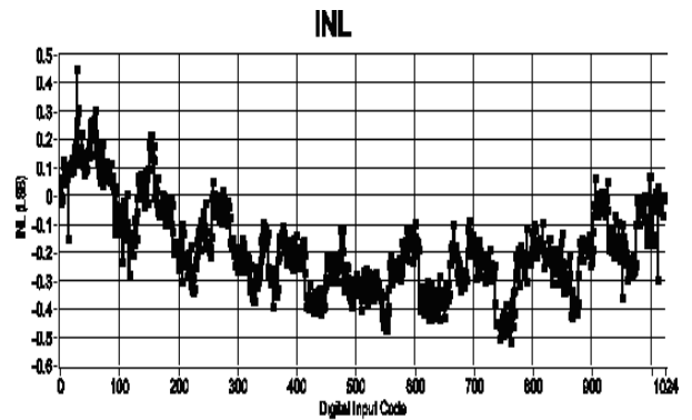
Figure 9. Typical INL
