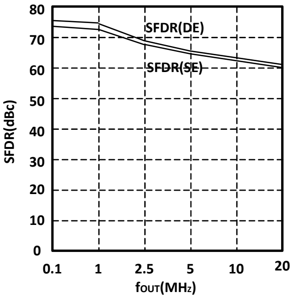
Figure 10. SFDR vs. f_{OUT} @ f_{CLK} = 50 MHz (Single-Ended and Differential-Ended)
