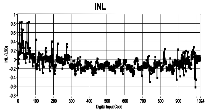
Figure 5. Typical INL
