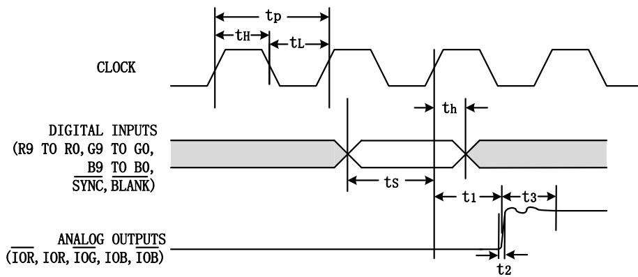
Figure 2. Timing Diagram
