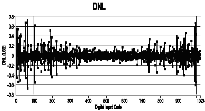
Figure 4. Typical DNL
