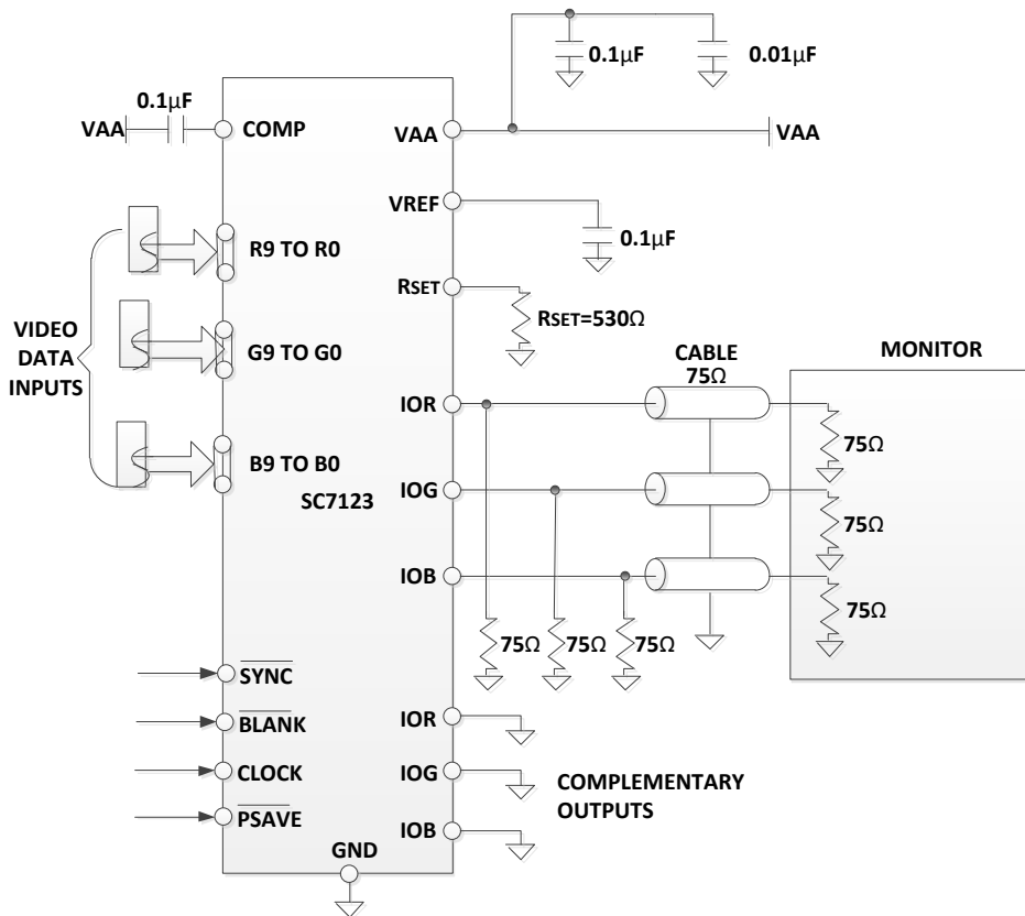
Figure17. Typical Connection Diagram
