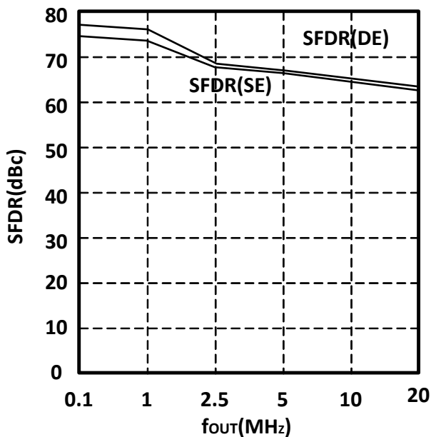
Figure 6. SFDR vs. f_{OUT} @ f_{CLK} = 50 MHz (Single-Ended and Differential-Ended)
