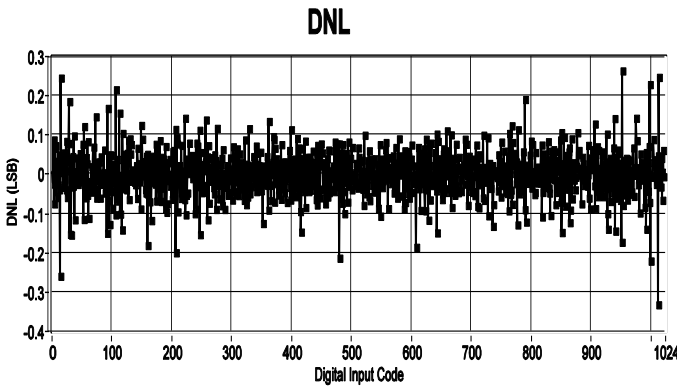
Figure 8. Typical DNL
